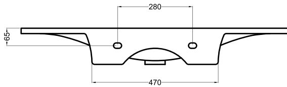
VISTA POSTERIORE REAR VIEW
